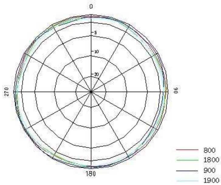
Vertical Pattern
